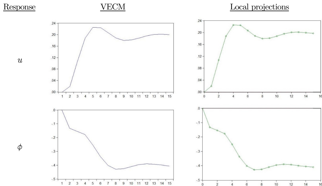
Figure 4: Impulse-response of u , \phi , and e to nonfactorized one standard deviation innovation in \omega .
