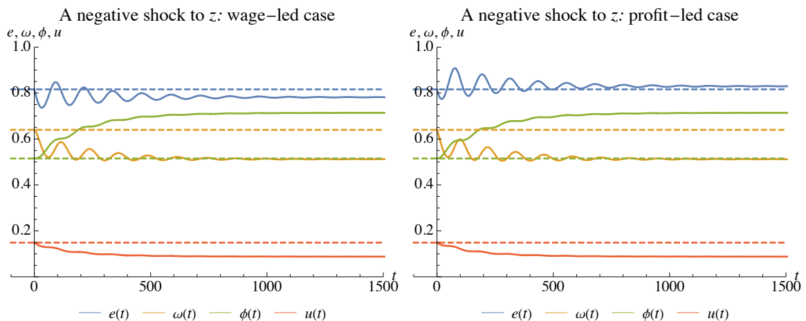
Figure 2: Simulations: a 5% time-zero reduction in z .
