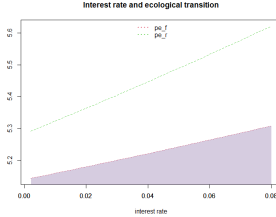
Figure 6.4: Economic system without CB intervention ( \frac{v_{er}}{v_{ef}} > 1 ; \frac{l_{er}}{l_{ef}} > 1 )
