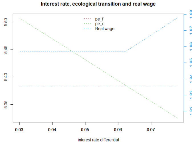
Figure 6.5: Ecological transition and real wage as the interest rate differential increase ( \frac{v_{er}}{v_{ef}} > 1 ; \frac{l_{er}}{l_{ef}} > 1 )
