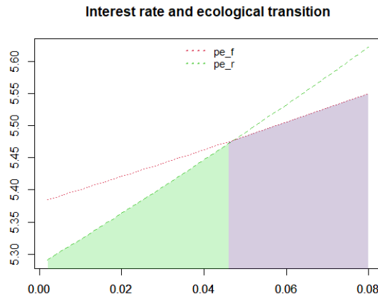
Figure 6.2: Price of renewable and fossil energy when the interest rate change ( \frac{v_{er}}{v_{ef}} > 1 ; \frac{l_{er}}{l_{ef}} < 1 )
