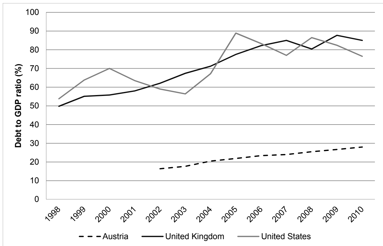
Figure 7: Ratio of mortgage debt to GDP in Austria, the United Kingdom and the United States
