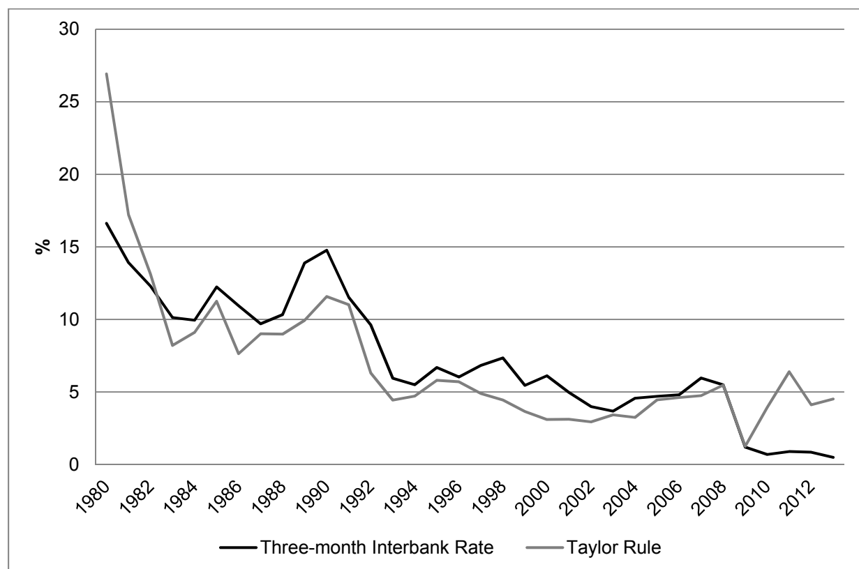
Figure 8: The United Kingdom's Three-Month Interbank Rate and Taylor Rule Prescriptions between 1980 and 2013 (%).
