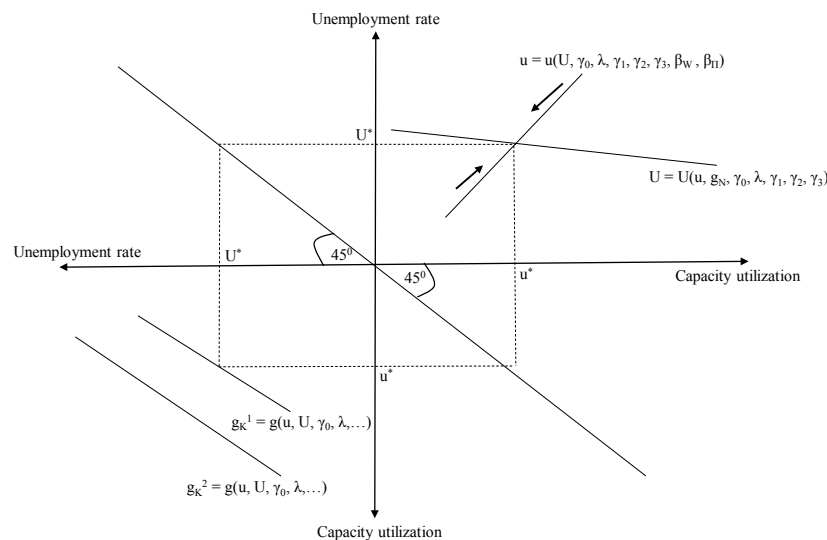
Figure 9. Determination of equilibrium in the extended profit-led neo-Kaleckian model with Kaldor – Hicks endogenous technological progress ( g_K^2 > g_K^1 ).
